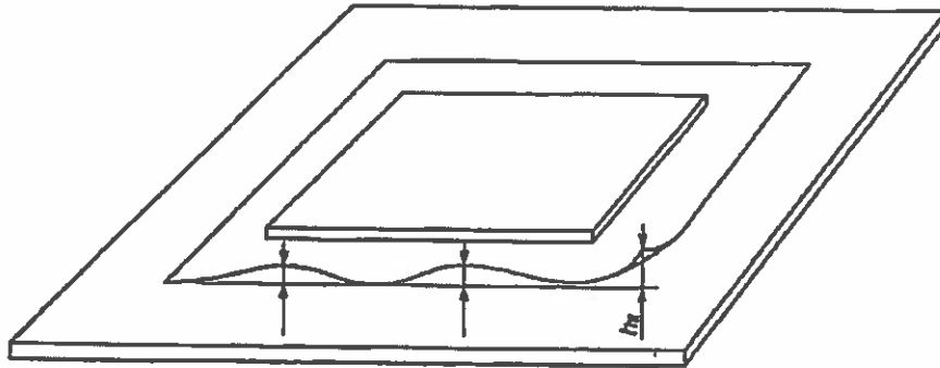
Figure 10 - Method of measuring centre fullness (indirect method)
