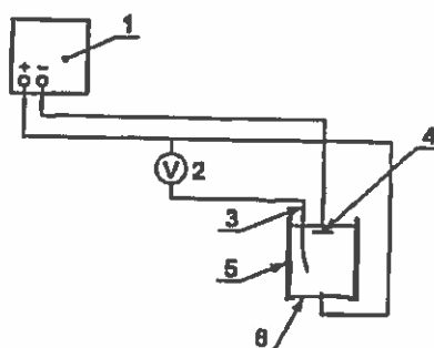
Figure E - 2 - Electro-stripping of chromium metal using the dual-purpose cell
